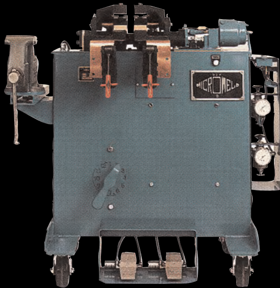
Models H & HX Steel Rod Butt Welders
